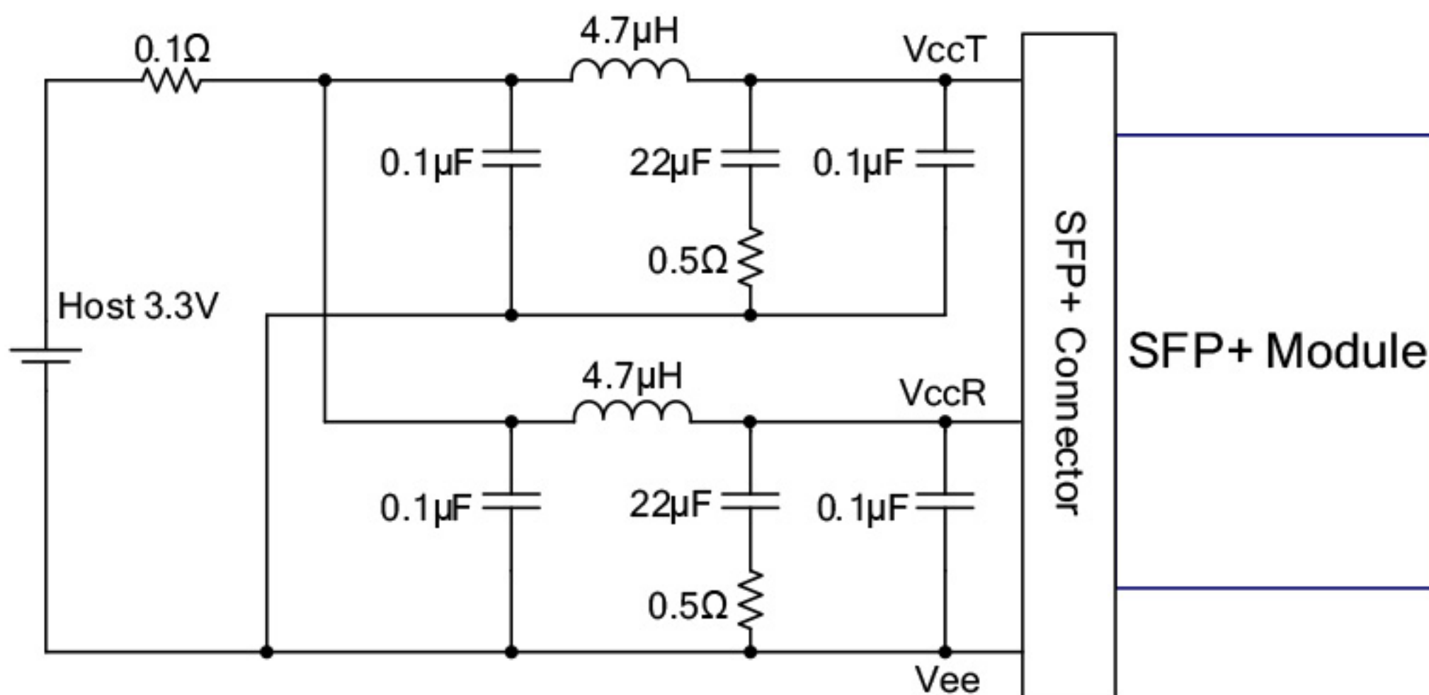
Figure2. Recommended Host Board Power Supply Filter Network
