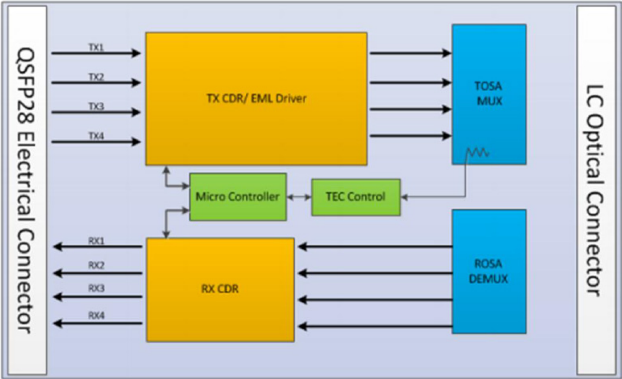
Figure1. Module Block Diagram
