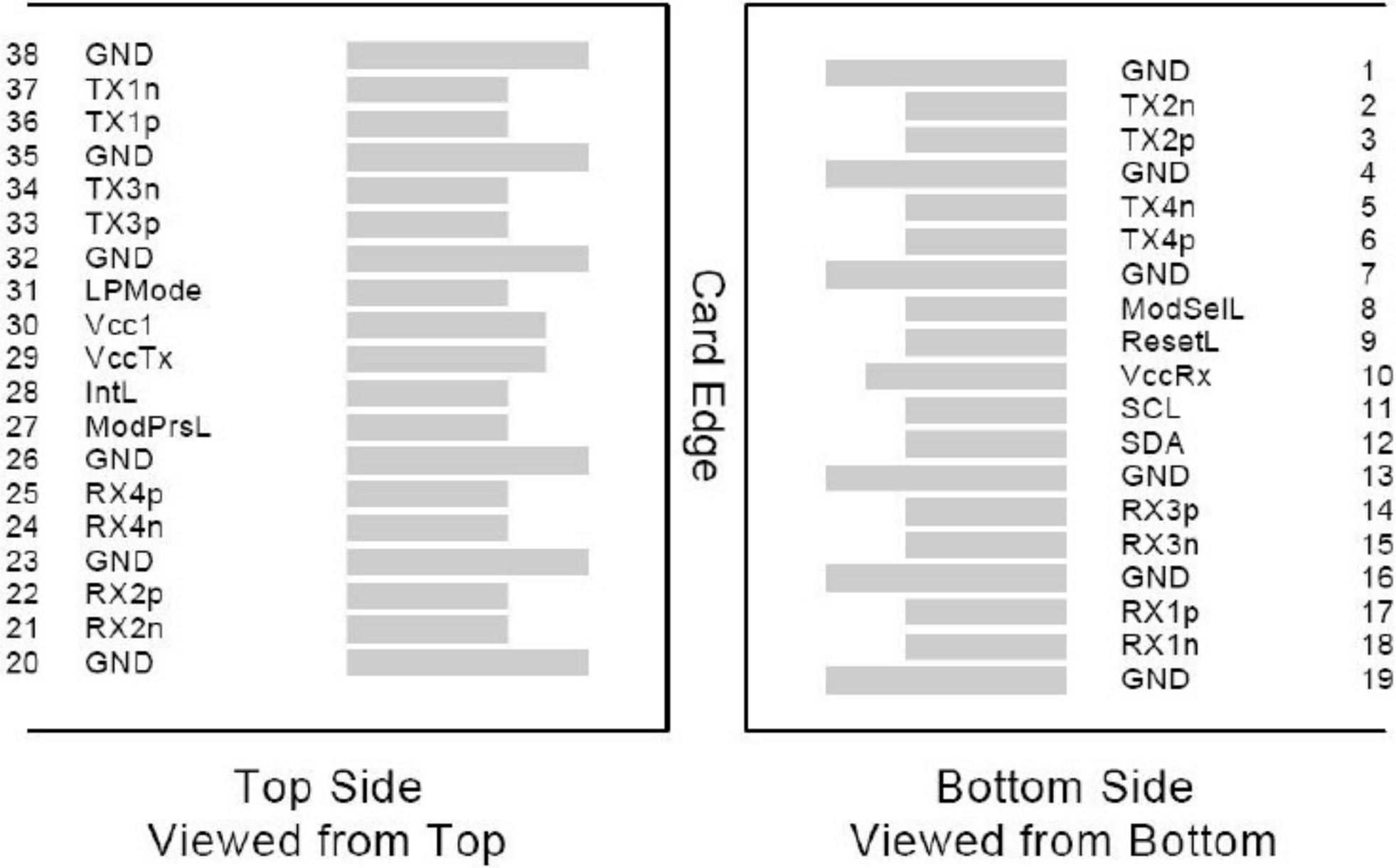
Figure3. Electrical Pin-out Details
