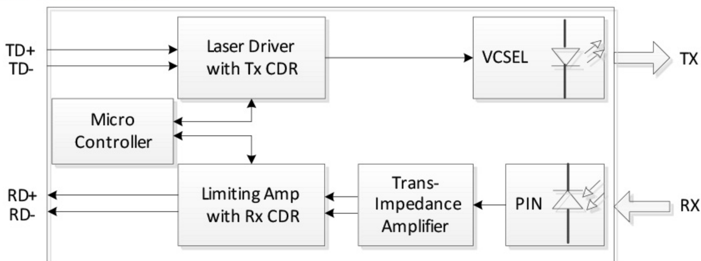
Figure 3: Transceiver Block Diagram
